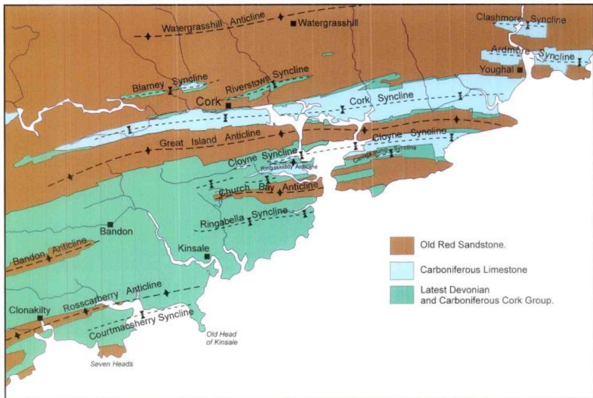
Figure 3. Geological setting of South Cork (after Sleeman and Pratch, 1994). The bay is underlain by Carboniferous Limestone, deposited between 355 and 290 million years ago, which controls the bay's configuration through inward erosion.
