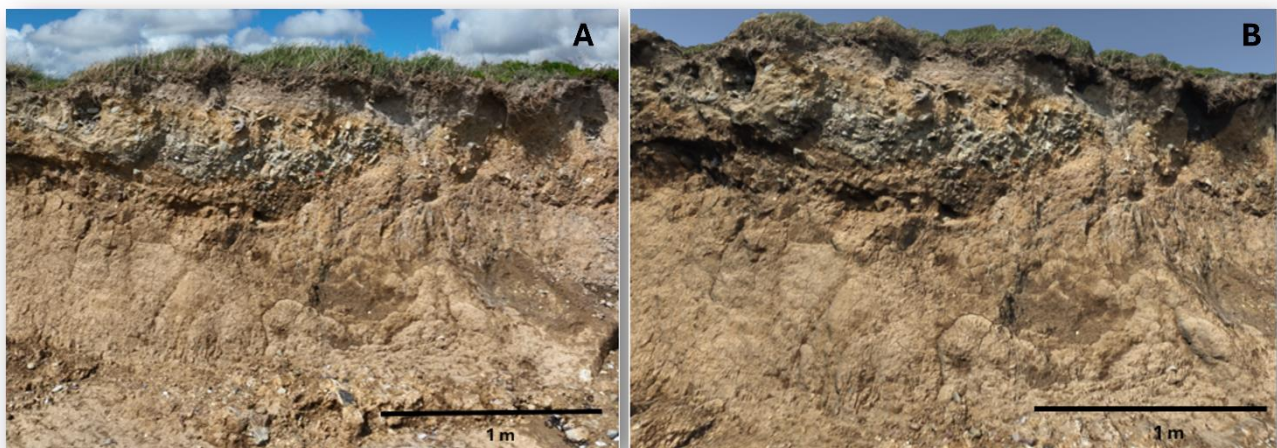
Figure 5. The two pictures show a section of the sea cliff at Garryvoe at a 1m scale. Picture A was taken during the survey, while picture B shows the 3D model of the same section generated on Agisoft. This appears to retain a high level of surface detail from the cliff.
