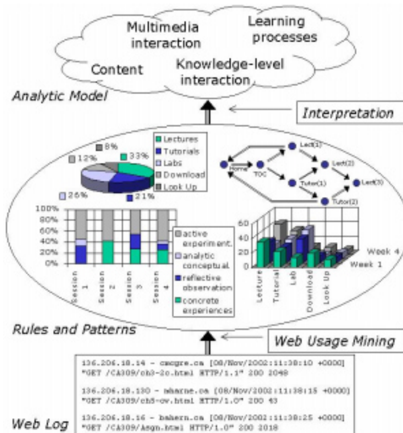
Figure 1. Web Usage Mining and Interpretation Architecture.
