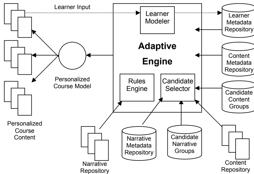
Fig. 1. Adaptive Hypermedia Service Architecture
