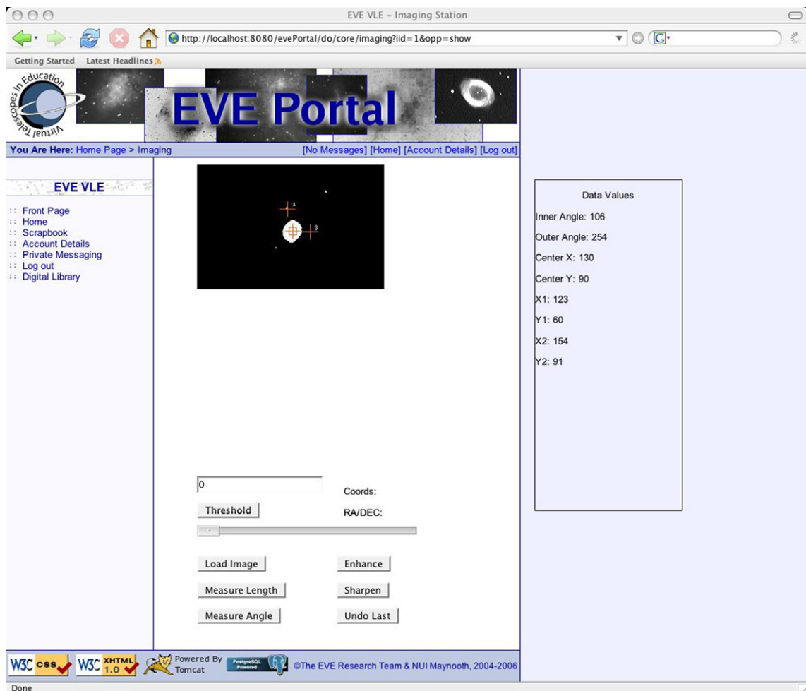
Fig. 5. Position angle change of Titan to Saturn.
