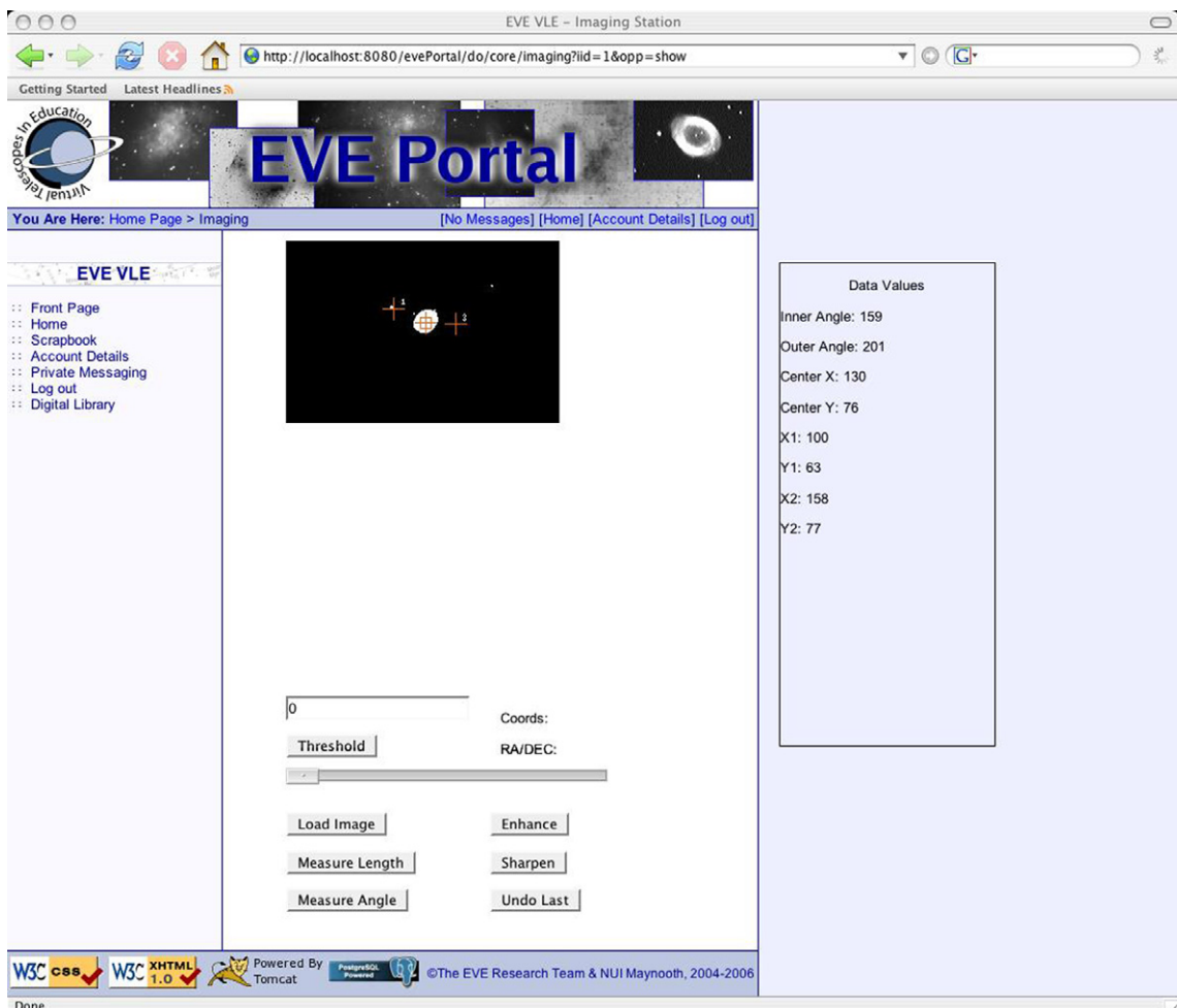
Fig. 4. Position angle of Titan to Saturn.
