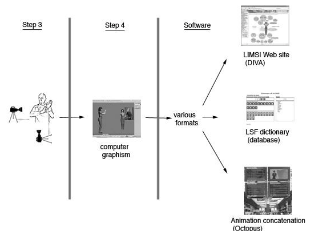
Figure 3: methodology 2/2
