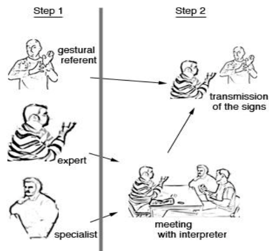
Figure 2: methodology 1/2
