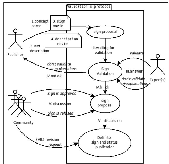
Figure 2: UML Case of utilisation: Validation system
