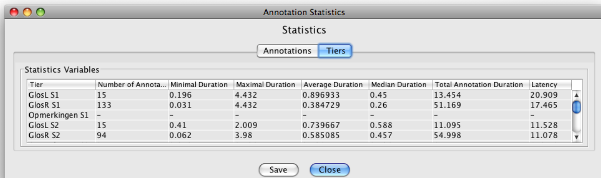
Figure 1. Tier statistics
